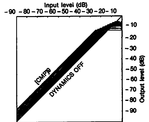
Input/output characteristics of compressor
