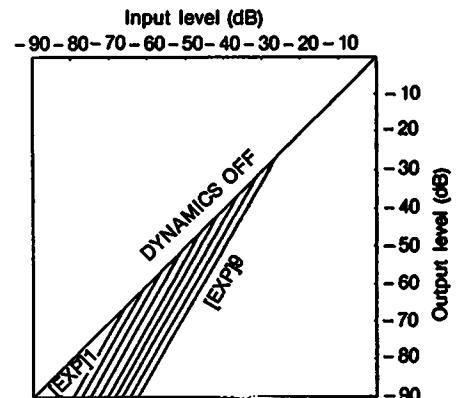
Input/output characteristics of expander
